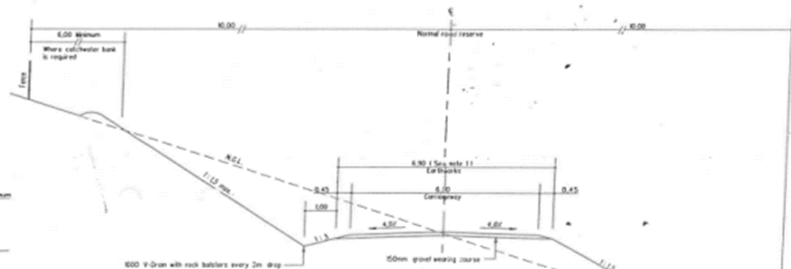
TYPE 6 DISTRICT ROAD (MOUNTAINOUS TERRAIN)
