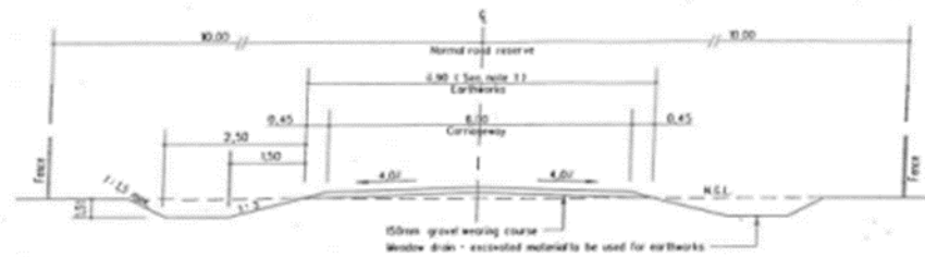
TYPE 6 DISTRICT ROAD (FLAT TERRAIN)
