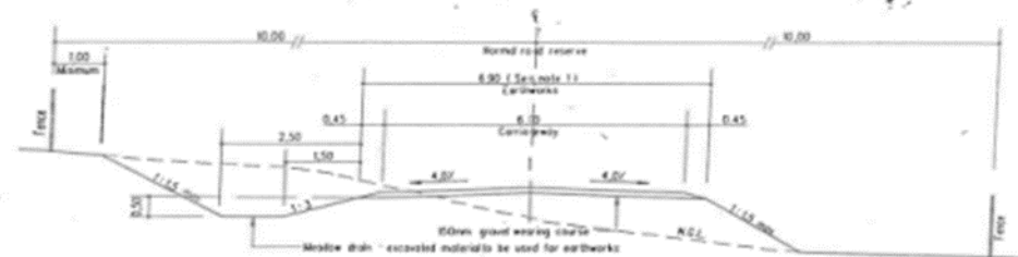
TYPE 6 DISTRICT ROAD (ROLLING TERRAIN)
